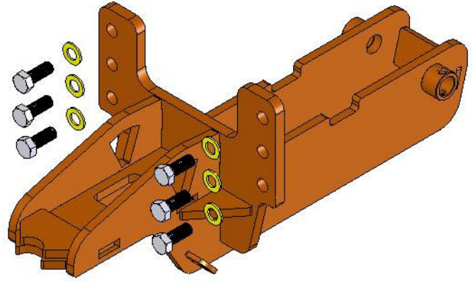
FRAME WITH BOLTS
