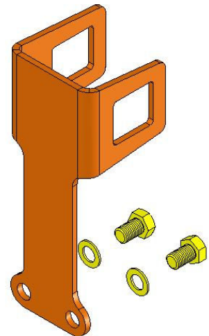
DRAWBAR POCKET KIT
