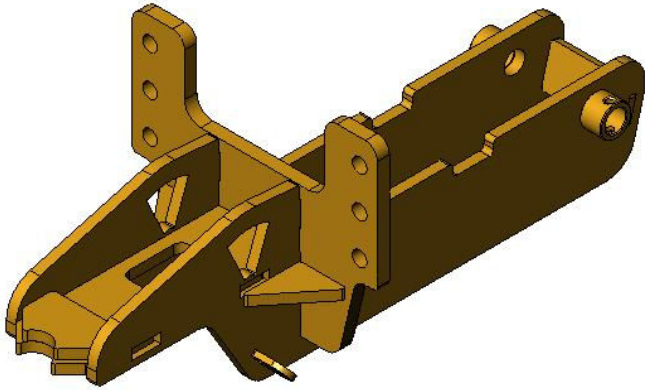
FRAME
