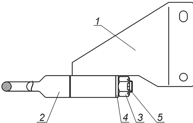
Fig. 6 Rotatable draught bar, full assembly
