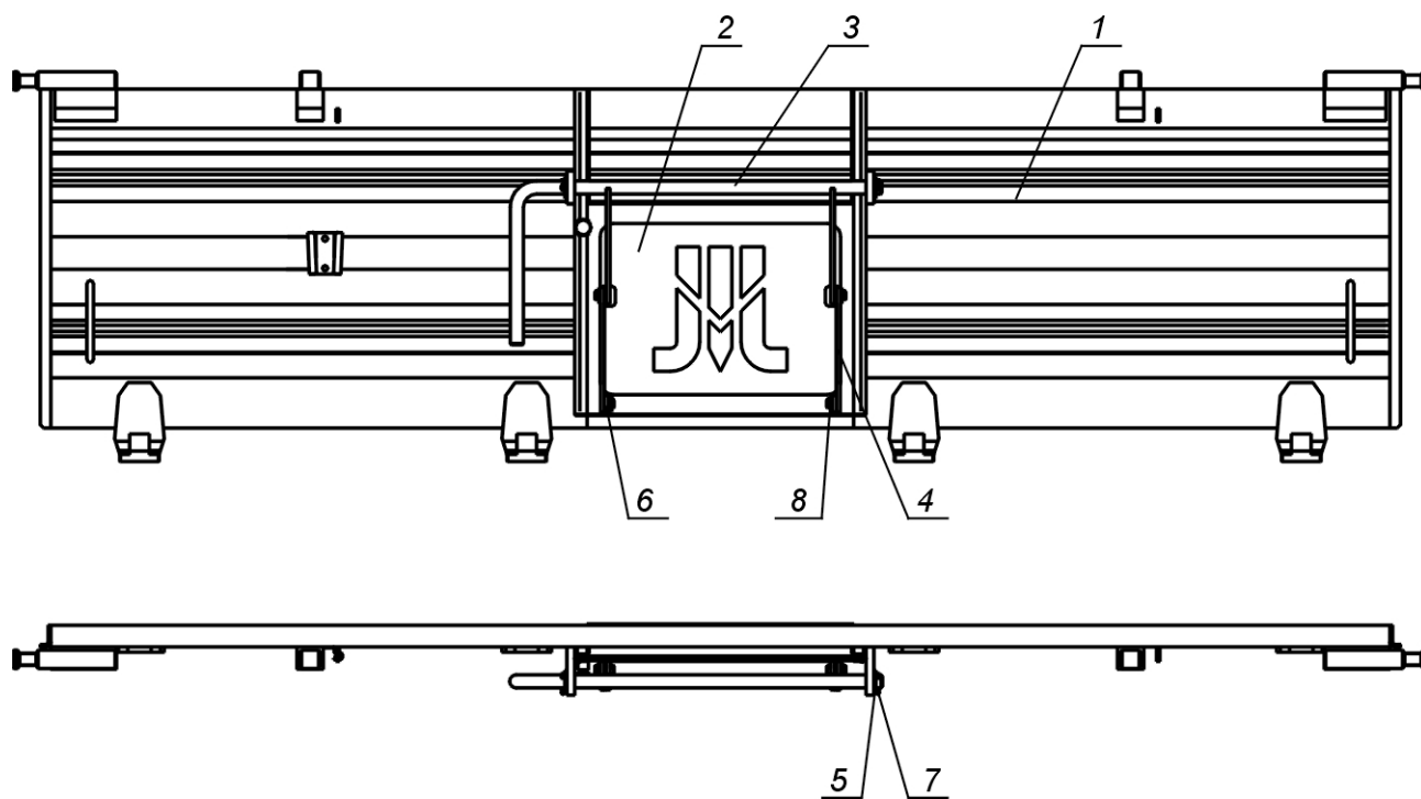
Fig. 22 FUHRMANN back wall
