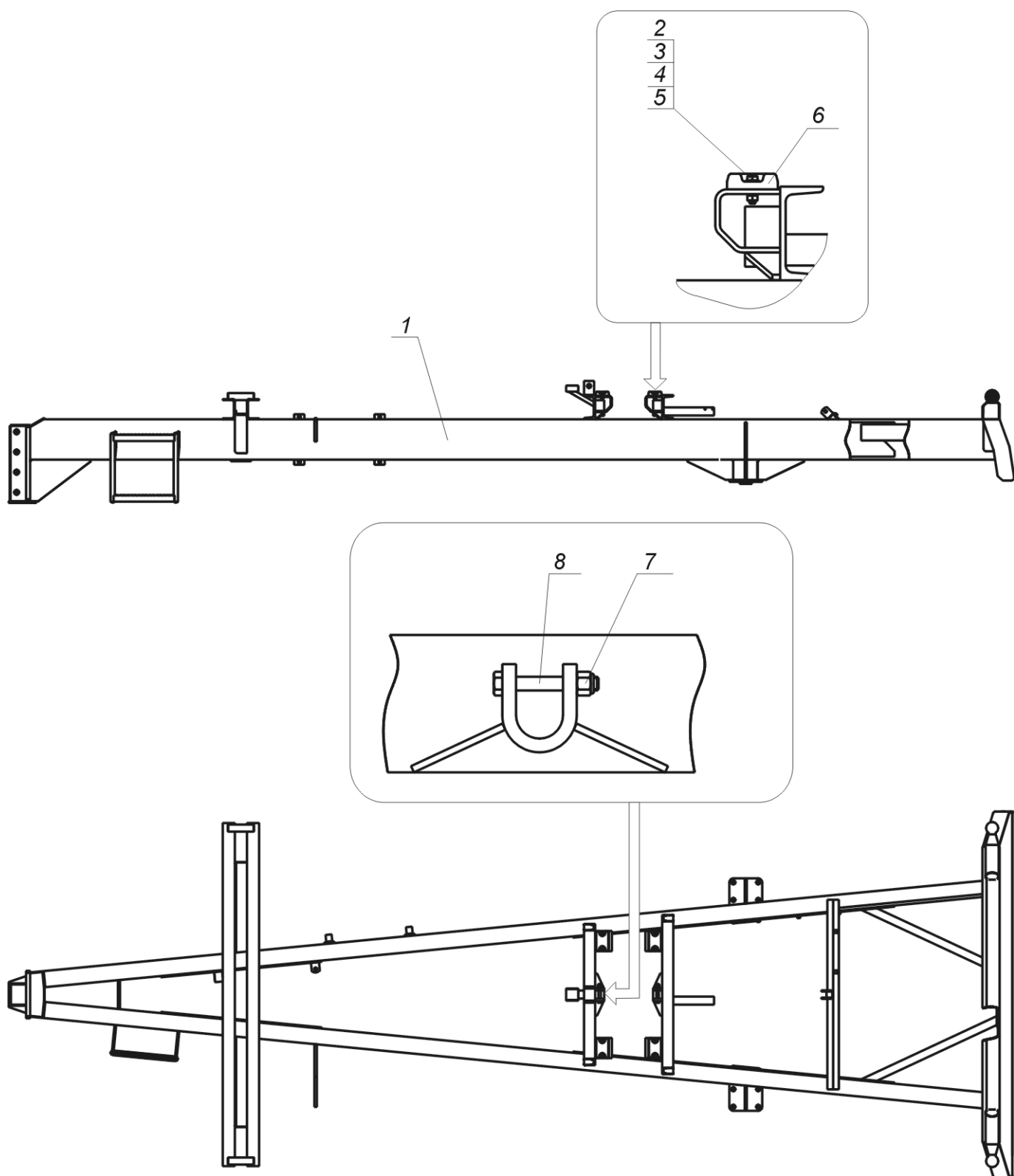
Fig. 4 Lower frame
