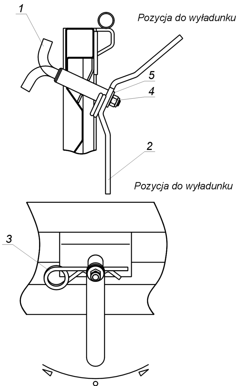
Fig. 26 Cord throwing out assembly, set
