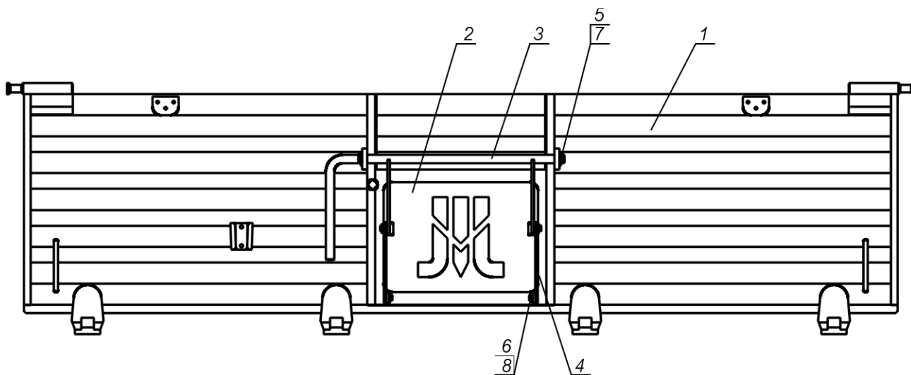
Fig. 20 PRONAR back wall
