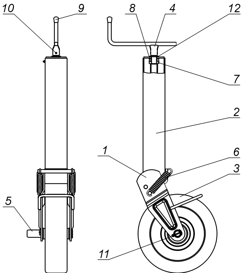
Fig. 30 Support with wheel, set
