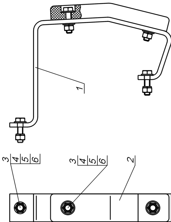
Fig. 28 Guard rail, set
