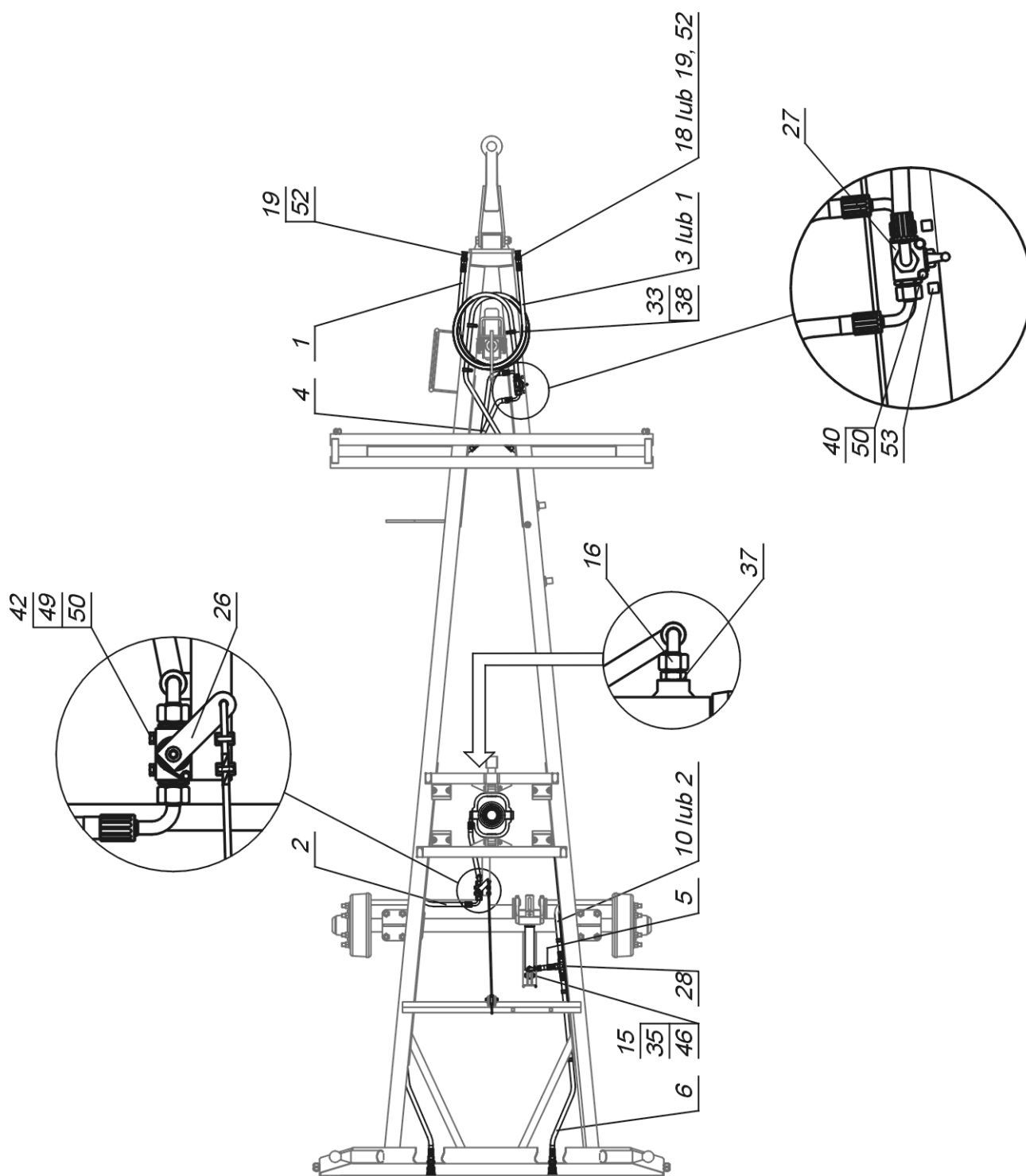
Fig. 10 Hydraulic system, top view
