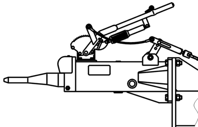
Fig. 36 Draught bar with overrunning brake
