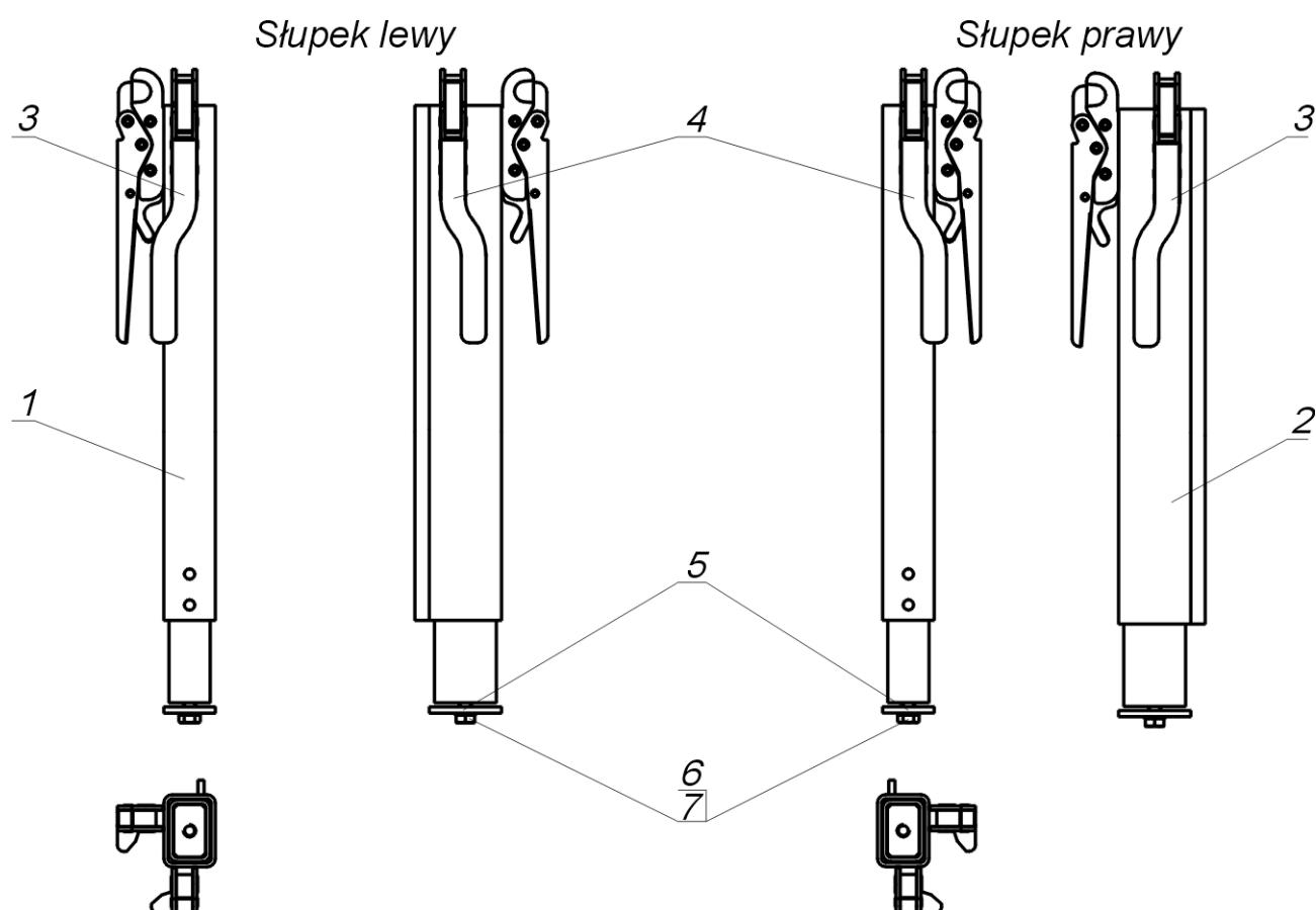
Fig. 23 FUHRMANN posts
