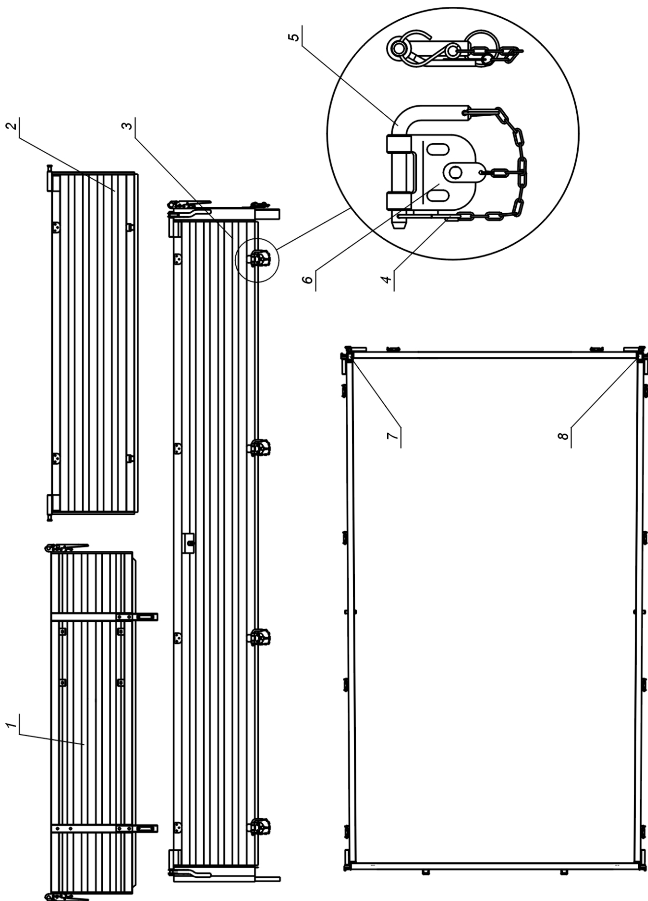
Fig. 14 PRONAR added top walls set
