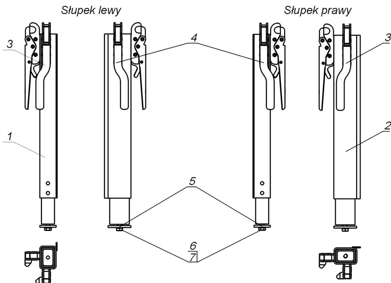
Fig. 21 PRONAR posts
