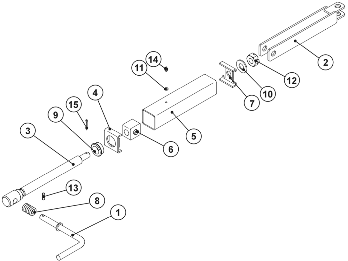
FIG. 38. BRAKE GEAR
