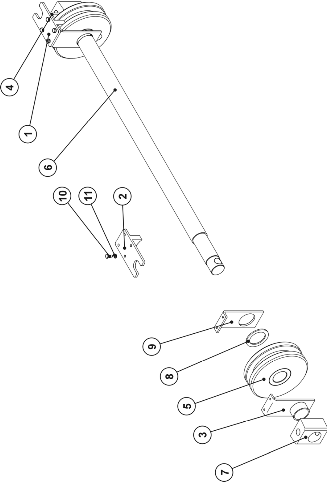
FIG. 4. FRONT AXLE
