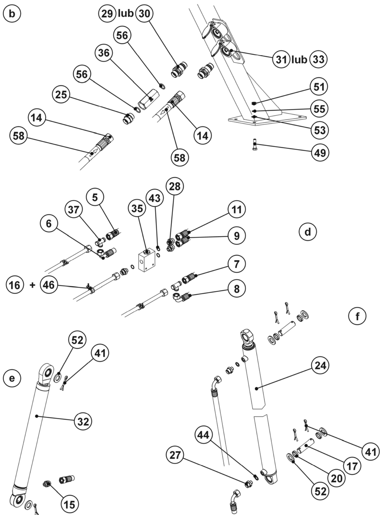
FIG. 33. HYDRAULIC SYSTEM
