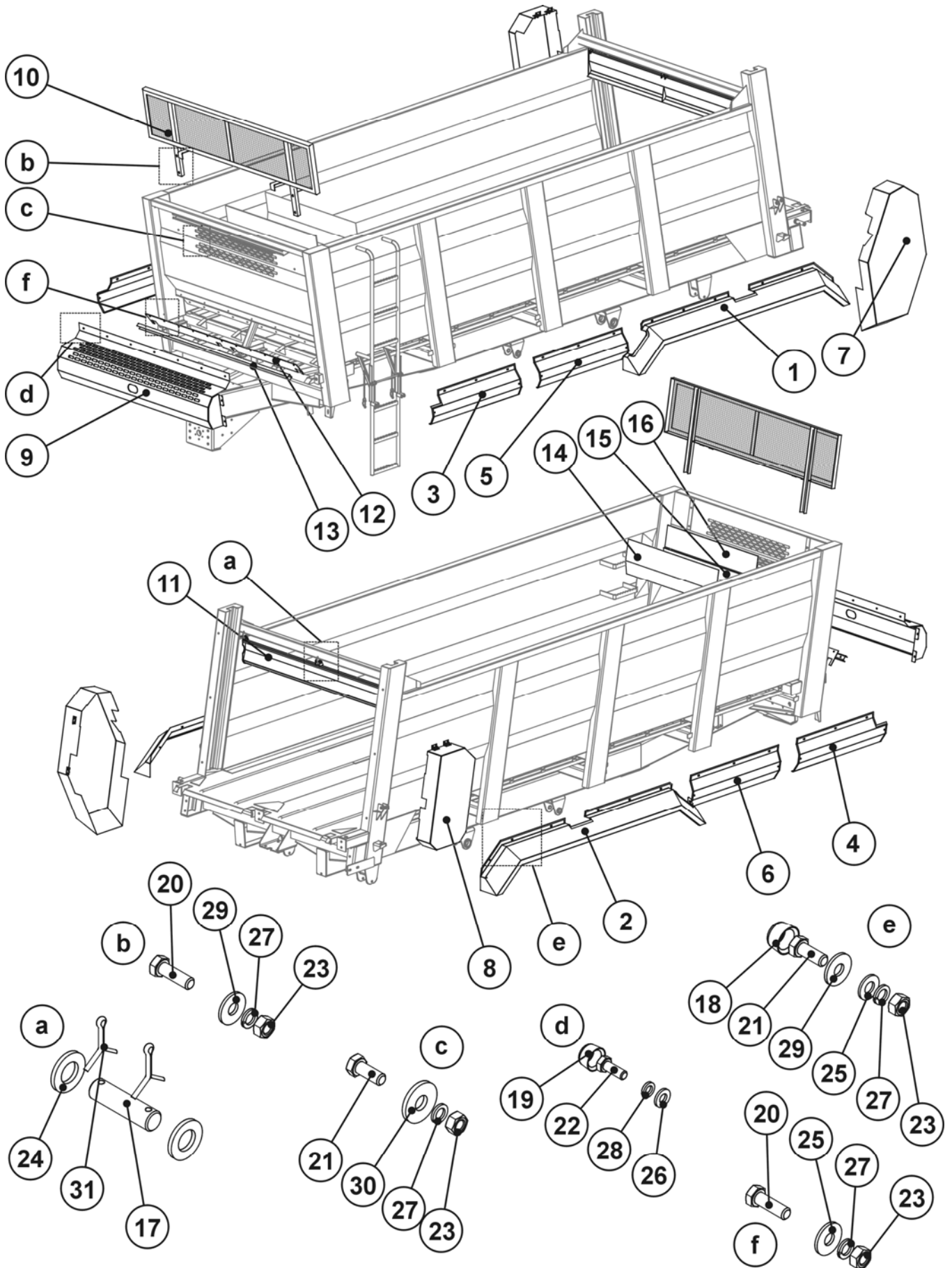
FIG. 2. GUARDS, CPL
