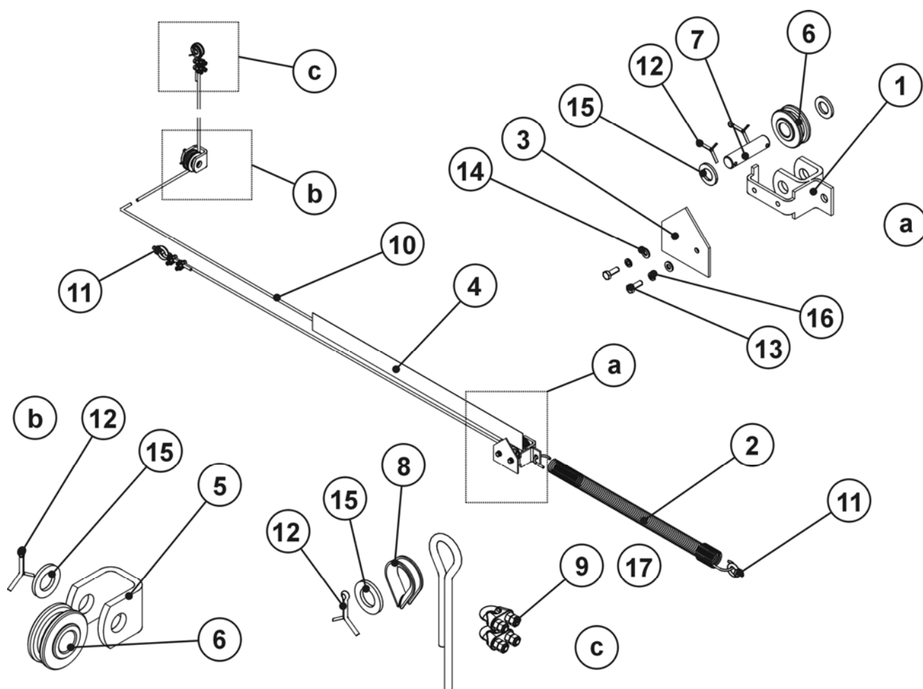
FIG. 47. GATE POSITION INDICATOR
