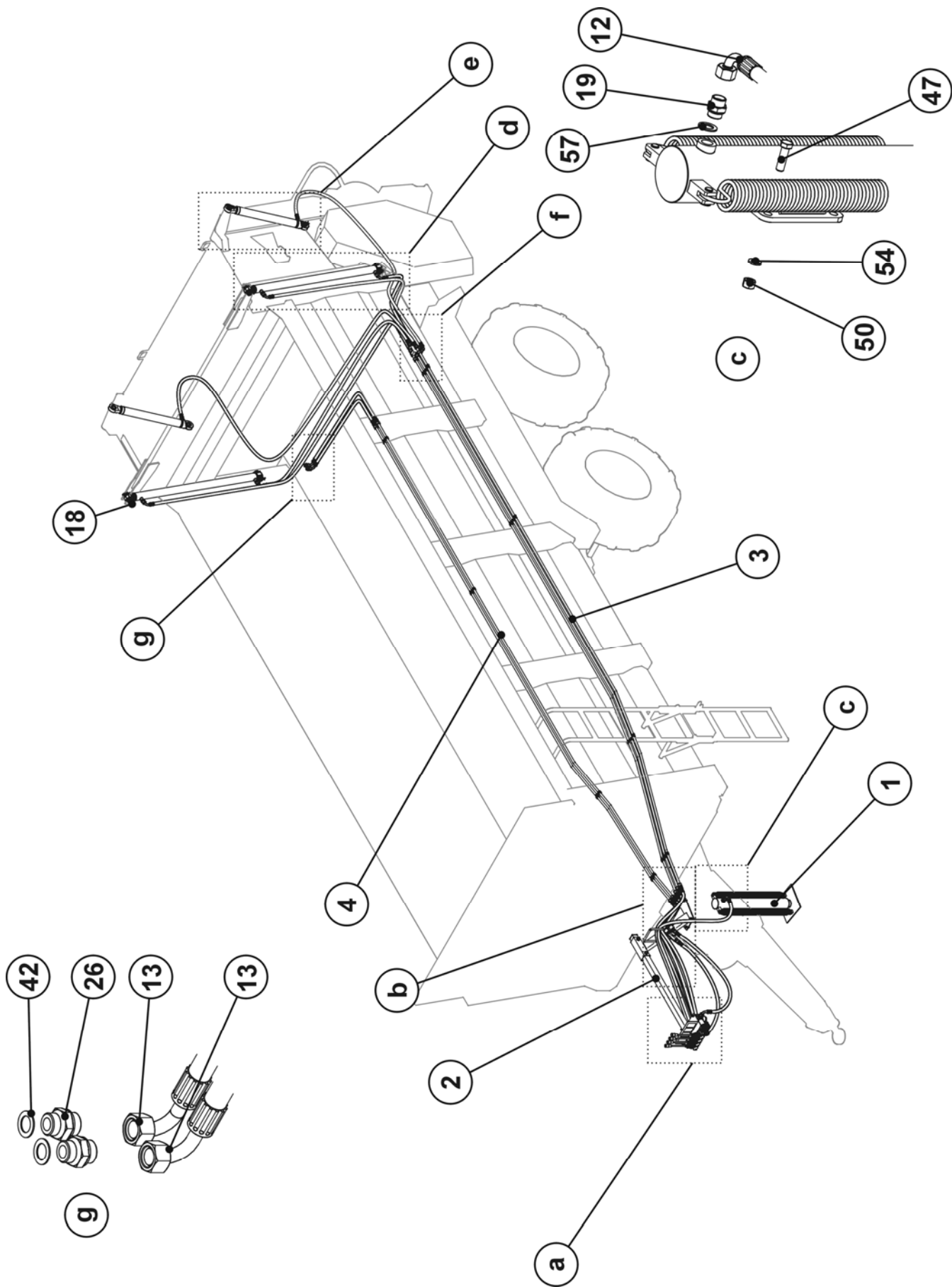
FIG. 31. HYDRAULIC SYSTEM
