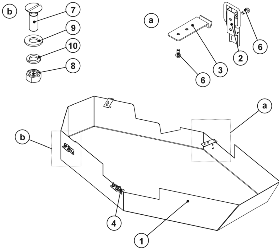
FIG. 29. LEFT ADAPTER GUARD
