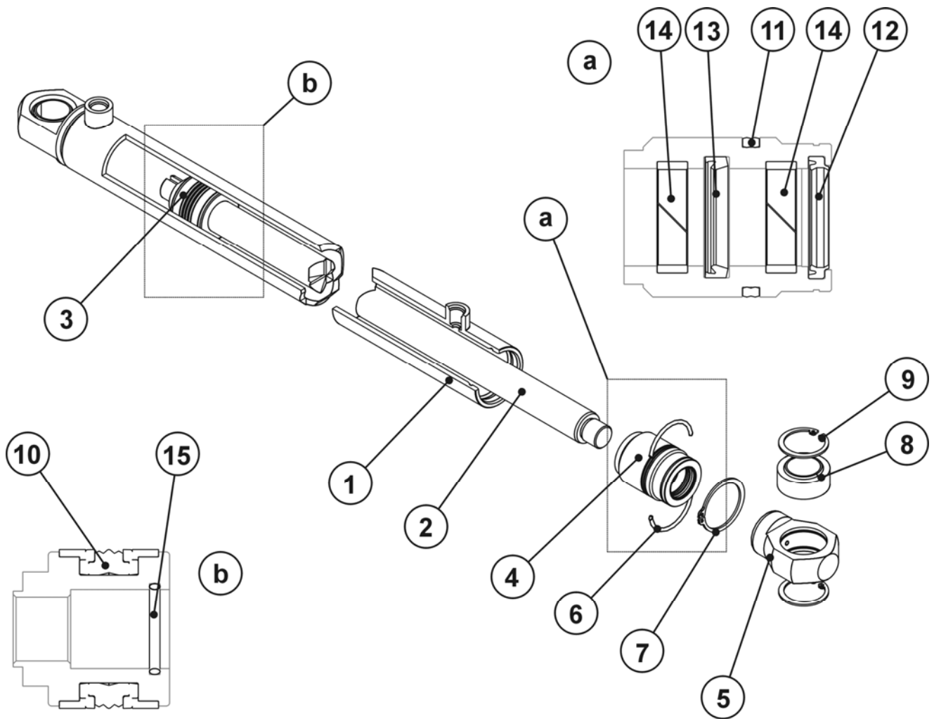
FIG. 35. CYLINDER
