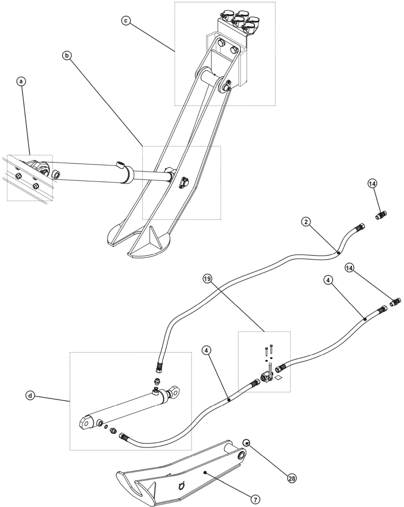
FIG. 25. SCISSOR SUPPORT HYDRAULIC SYSTEM
