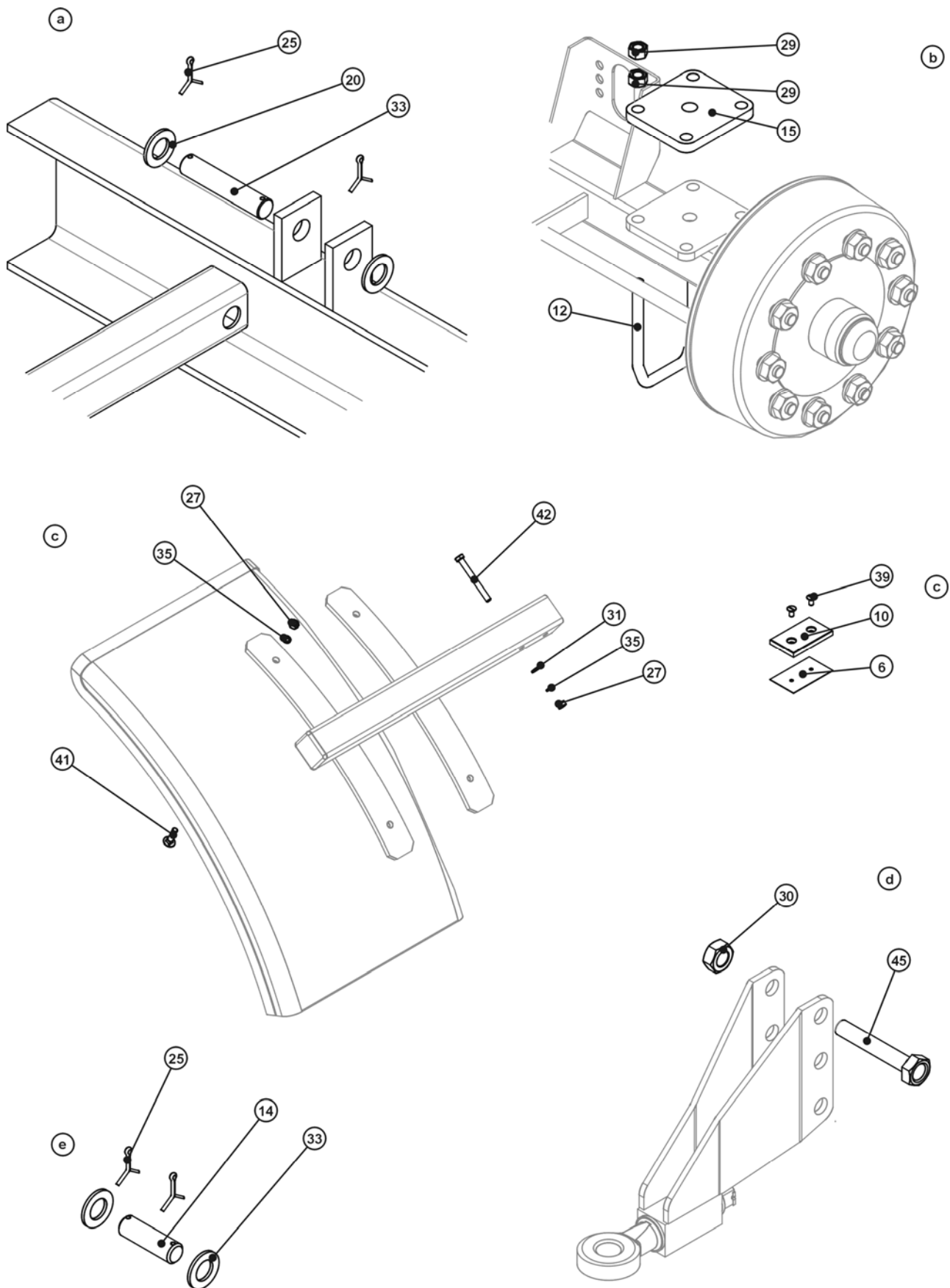
FIG. 2. UNDERCARRIAGE
