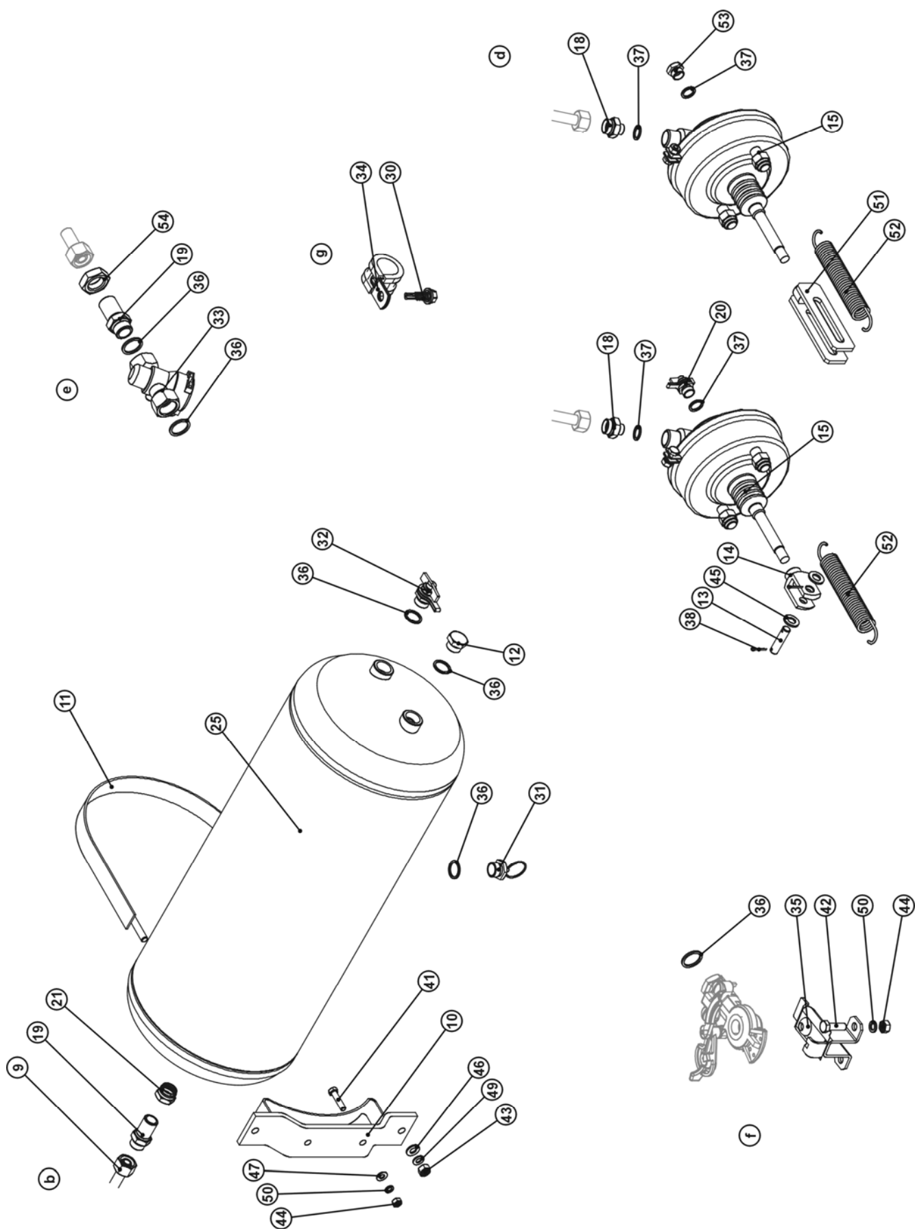
FIG. 11. PNEUMATIC BRAKE SYSTEM II WITH AUTOMATED CONTROLLER
