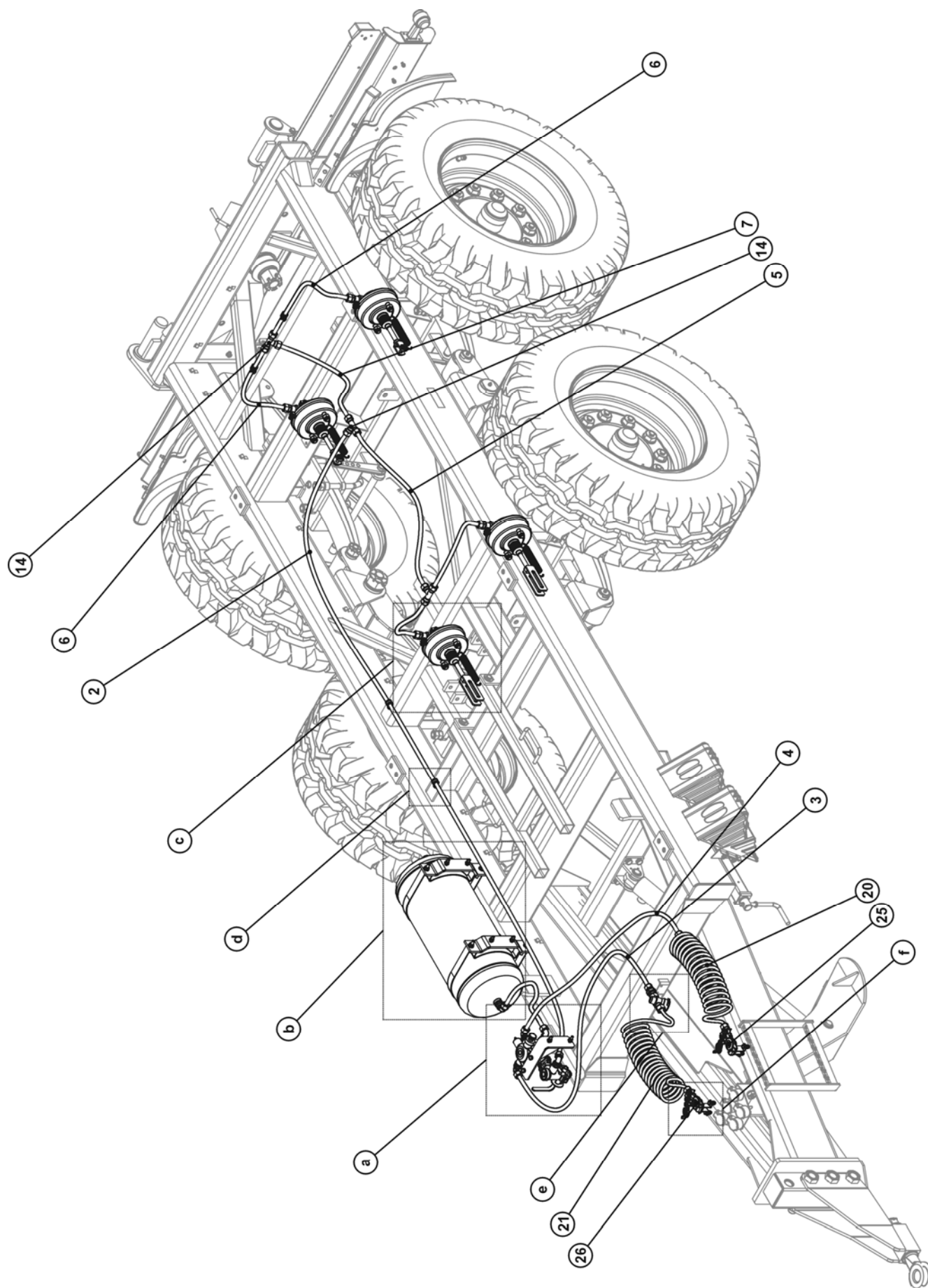
FIG. 16. DOUBLE-CONDUIT PNEUMATIC BRAKE SYSTEM II WITH THREE-RANGE CONTROLLER
