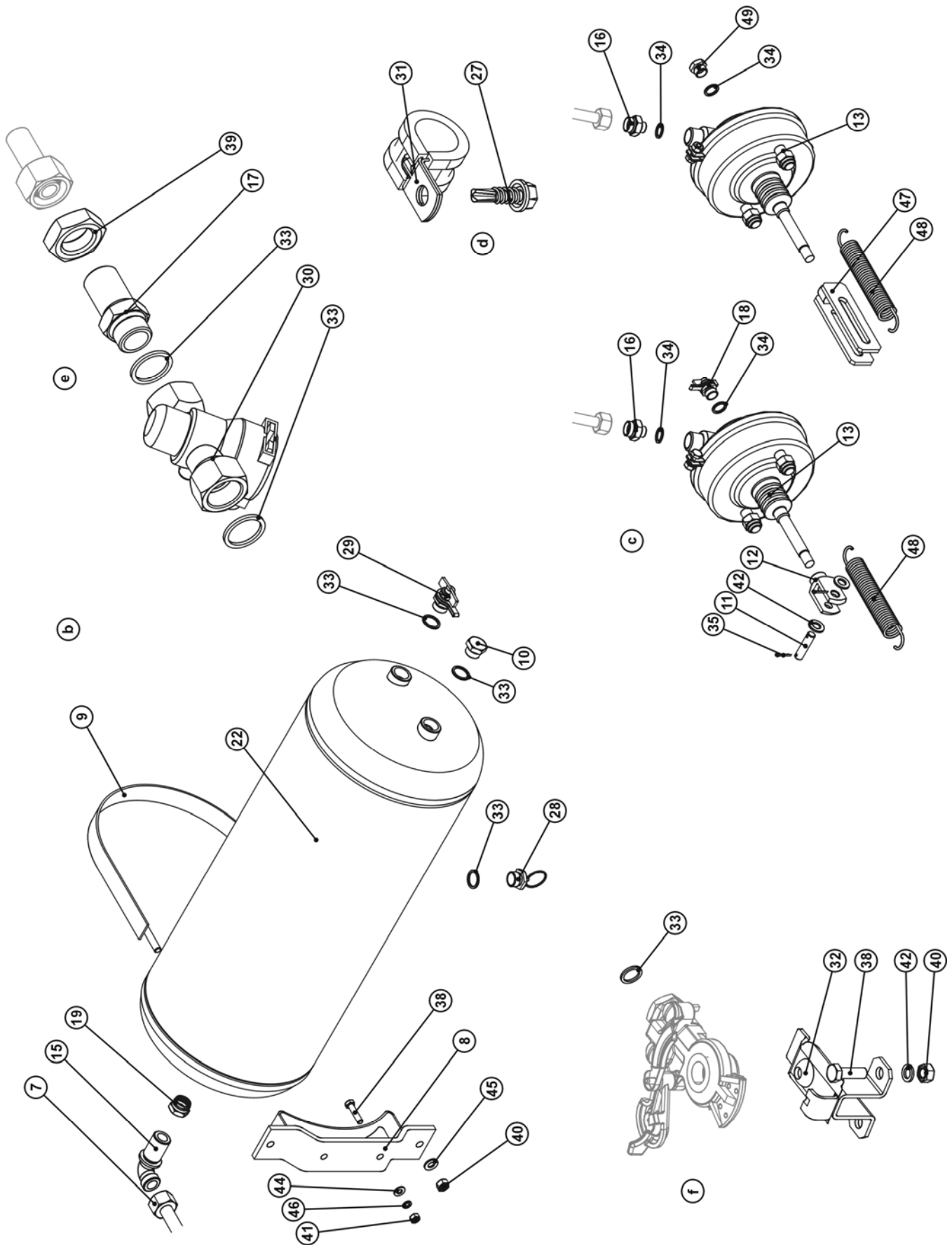
FIG. 17. DOUBLE-CONDUIT PNEUMATIC BRAKE SYSTEM I WITH THREE-RANGE CONTROLLER
