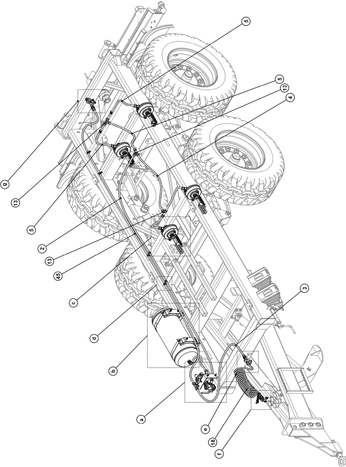
FIG. 19. SINGLE-CONDUIT PNEUMATIC BRAKE SYSTEM I WITH THREE-RANGE CONTROLLER
