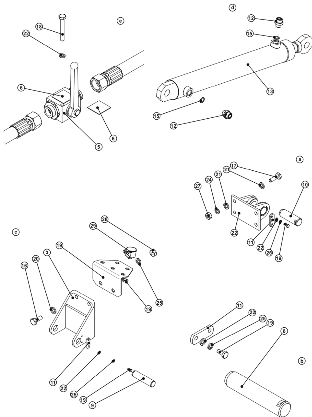
FIG. 26. SCISSOR SUPPORT HYDRAULIC SYSTEM
