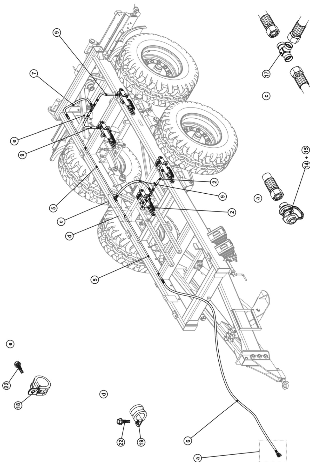
FIG. 30. HYDRAULIC BRAKE SYSTEM II
