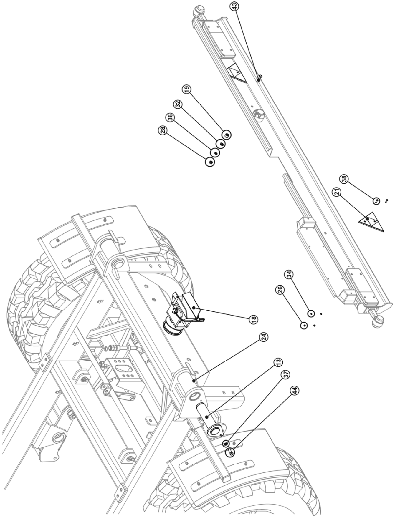
FIG. 3. UNDERCARRIAGE
