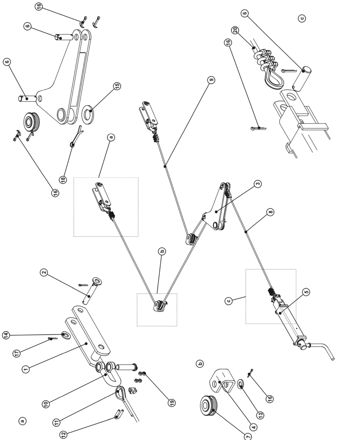
FIG. 38. PARKING BRAKE
