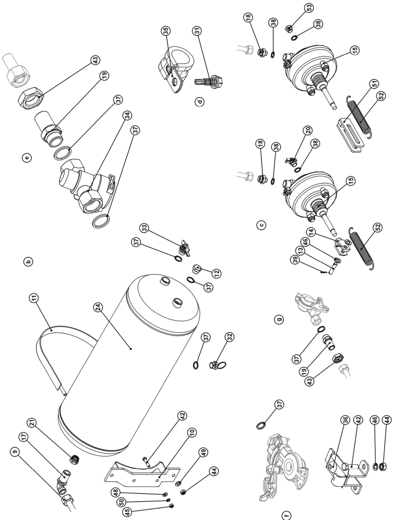
DOUBLE-CONDUIT PNEUMATIC BRAKE SYSTEM I WITH THREE-RANGE CONTROLLER
