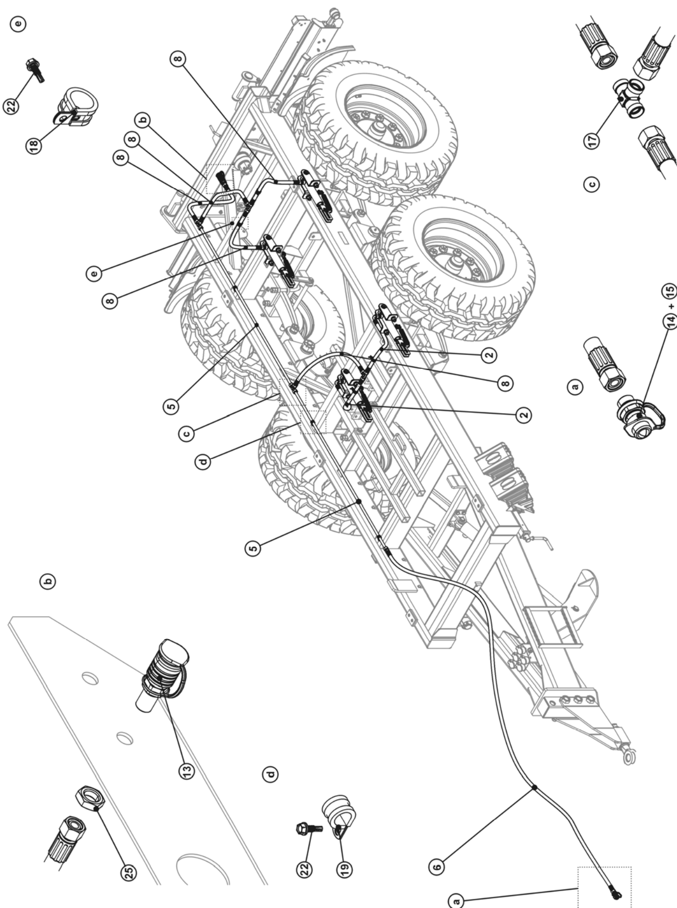
FIG. 28. HYDRAULIC BRAKE SYSTEM I
