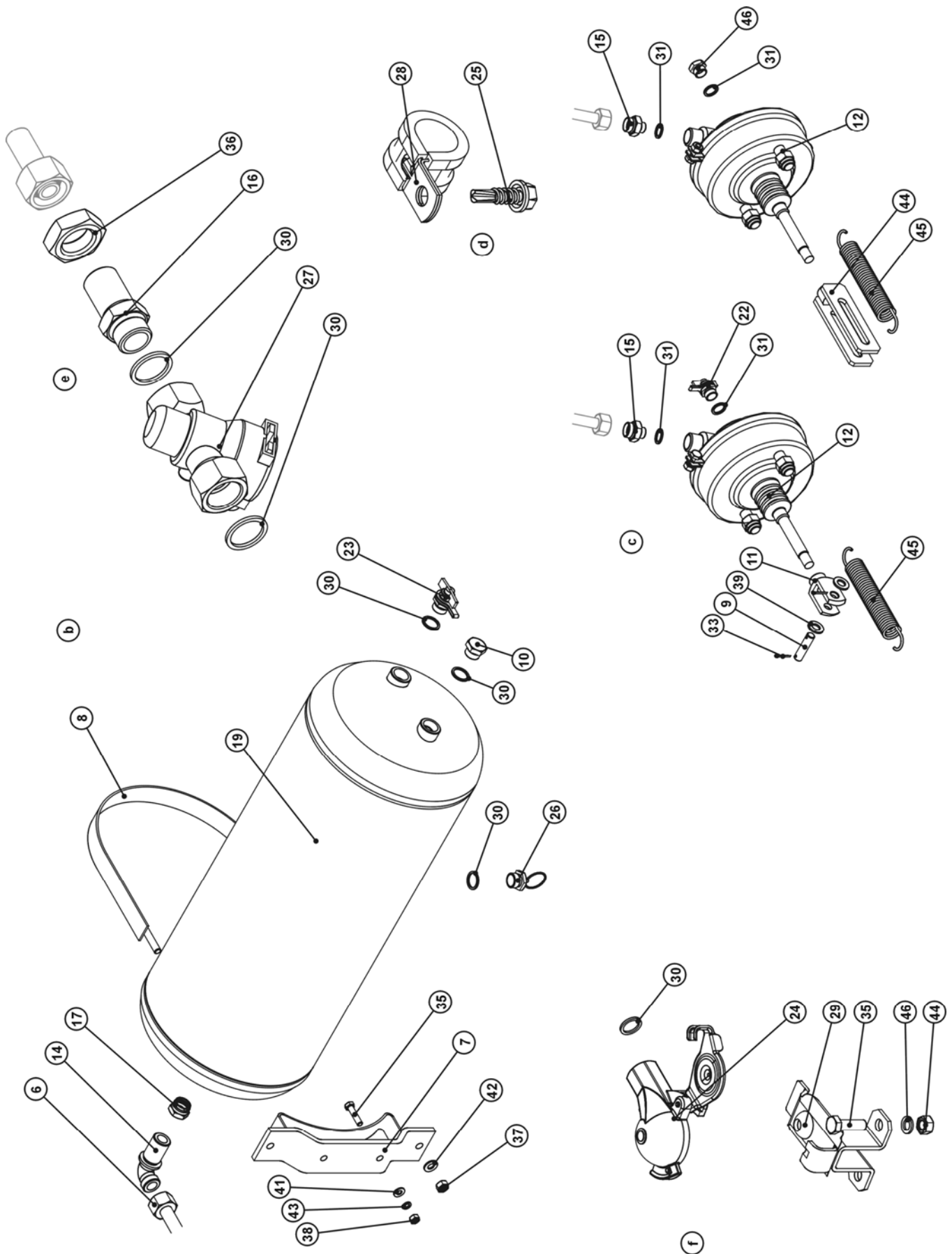
FIG. 23. SINGLE-CONDUIT PNEUMATIC BRAKE SYSTEM II WITH THREE-RANGE CONTROLLER
