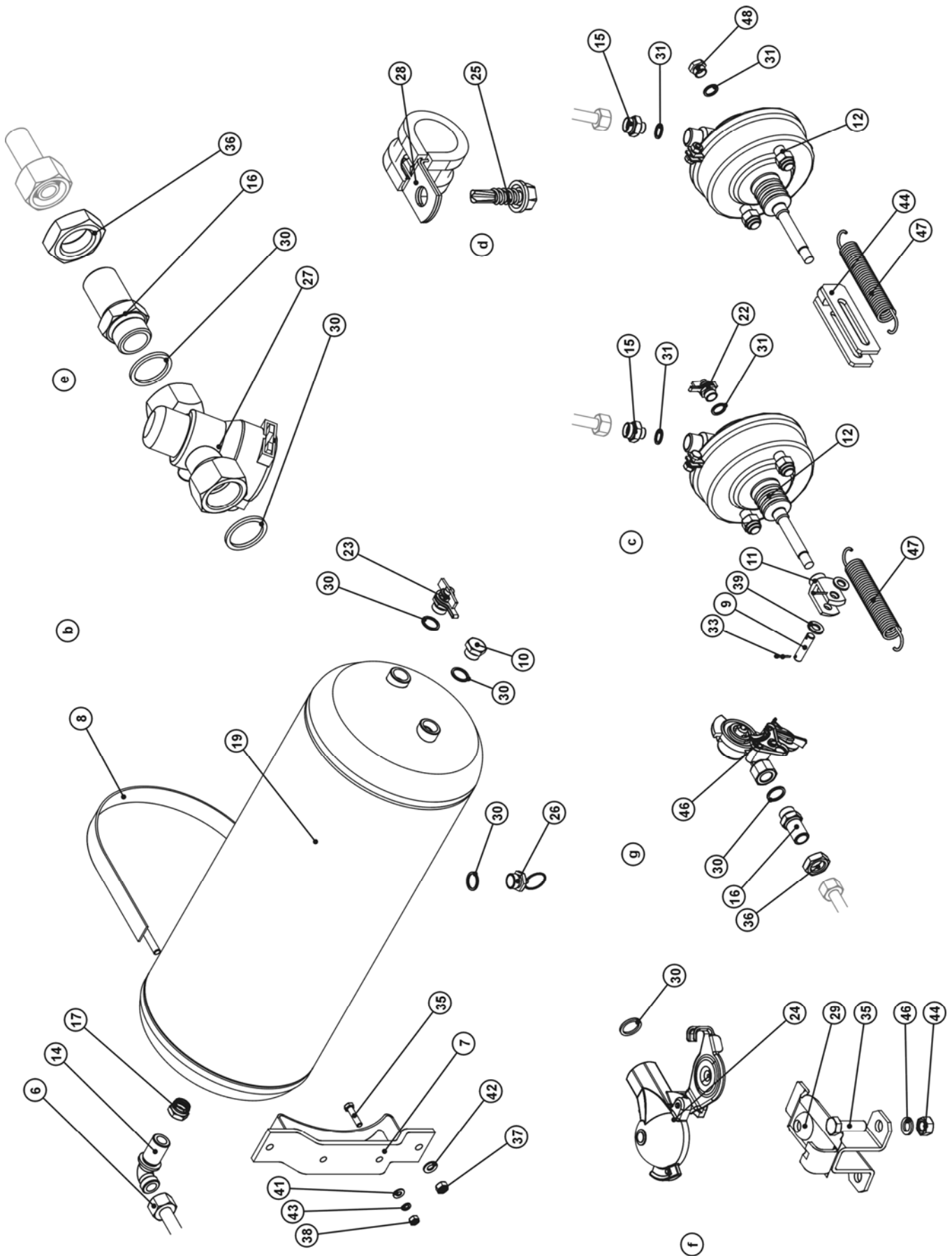
FIG. 20. SINGLE-CONDUIT PNEUMATIC BRAKE SYSTEM I WITH THREE-RANGE CONTROLLER
