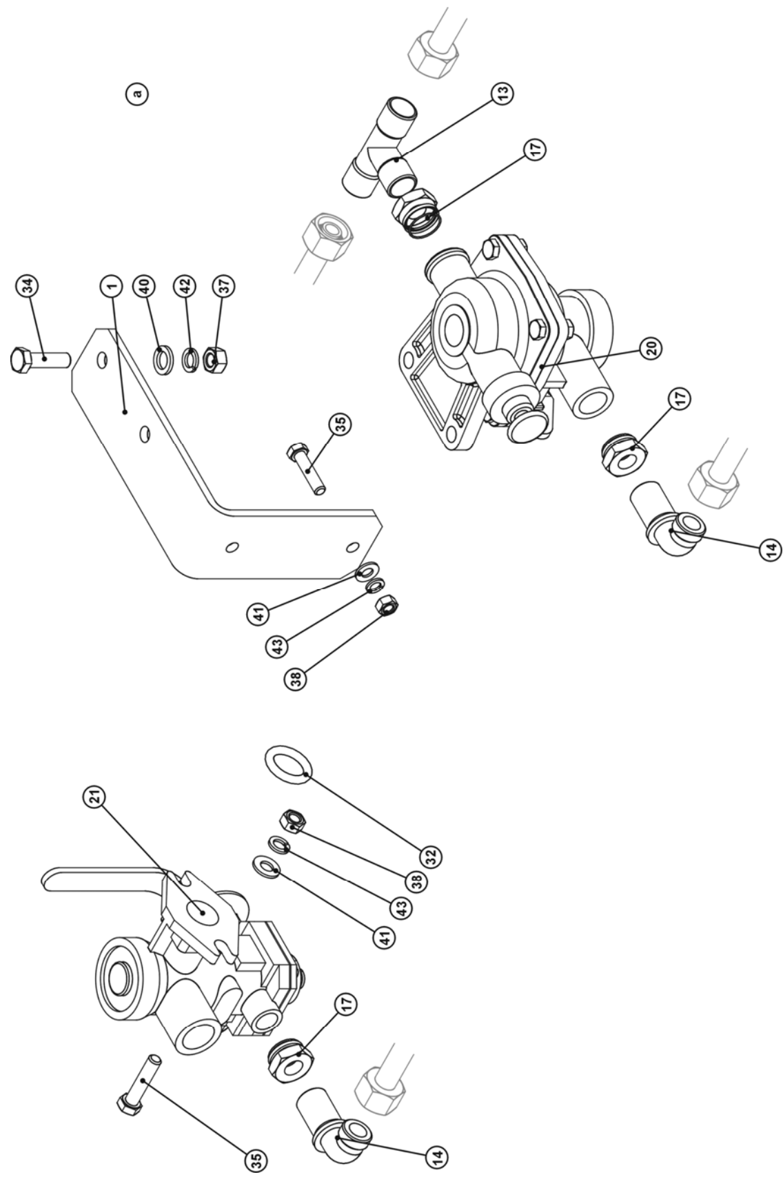
FIG. 21. SINGLE-CONDUIT PNEUMATIC BRAKE SYSTEM I WITH THREE-RANGE CONTROLLER
