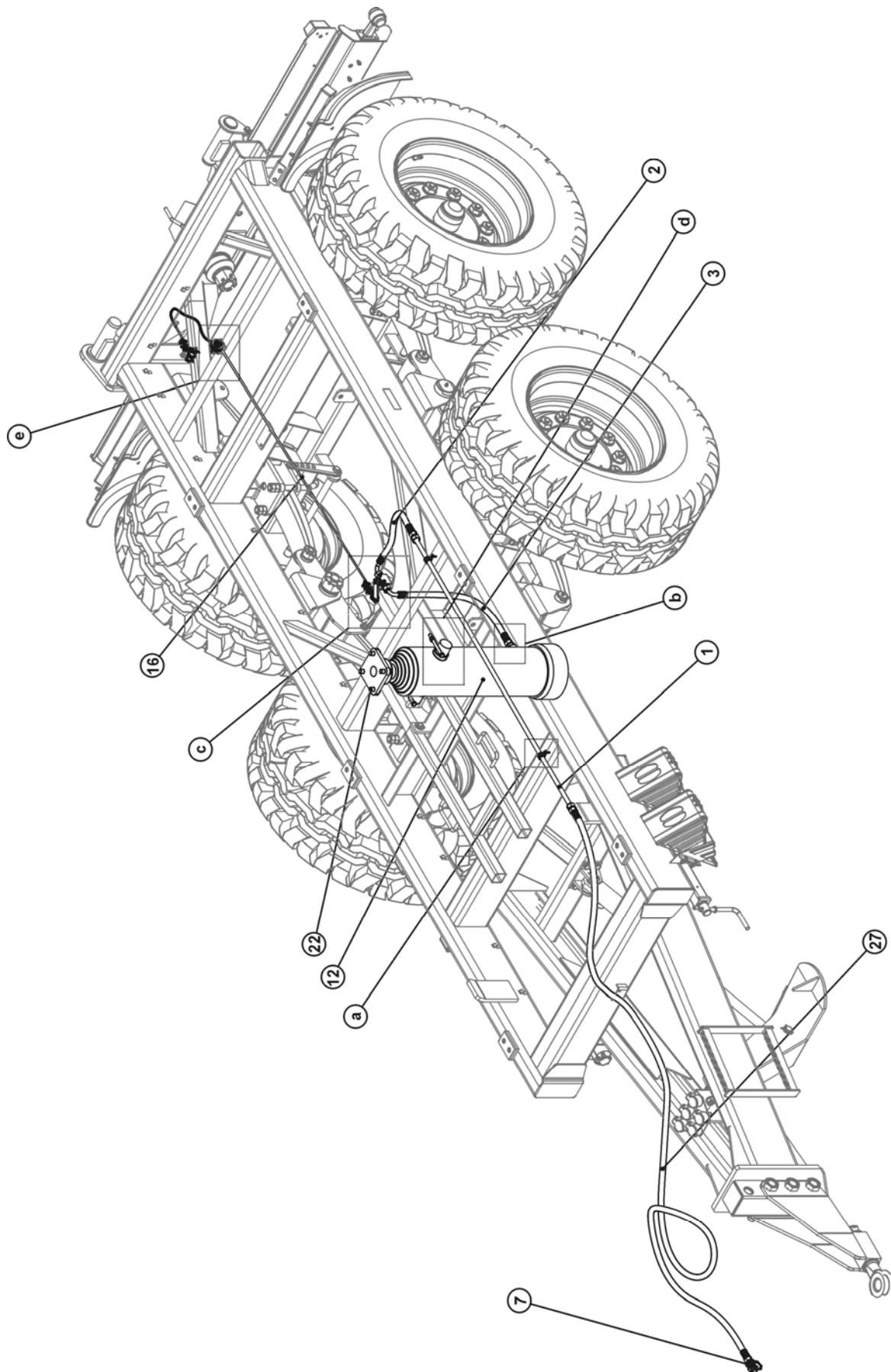
FIG. 35. HYDRAULIC TILTING SYSTEM II
