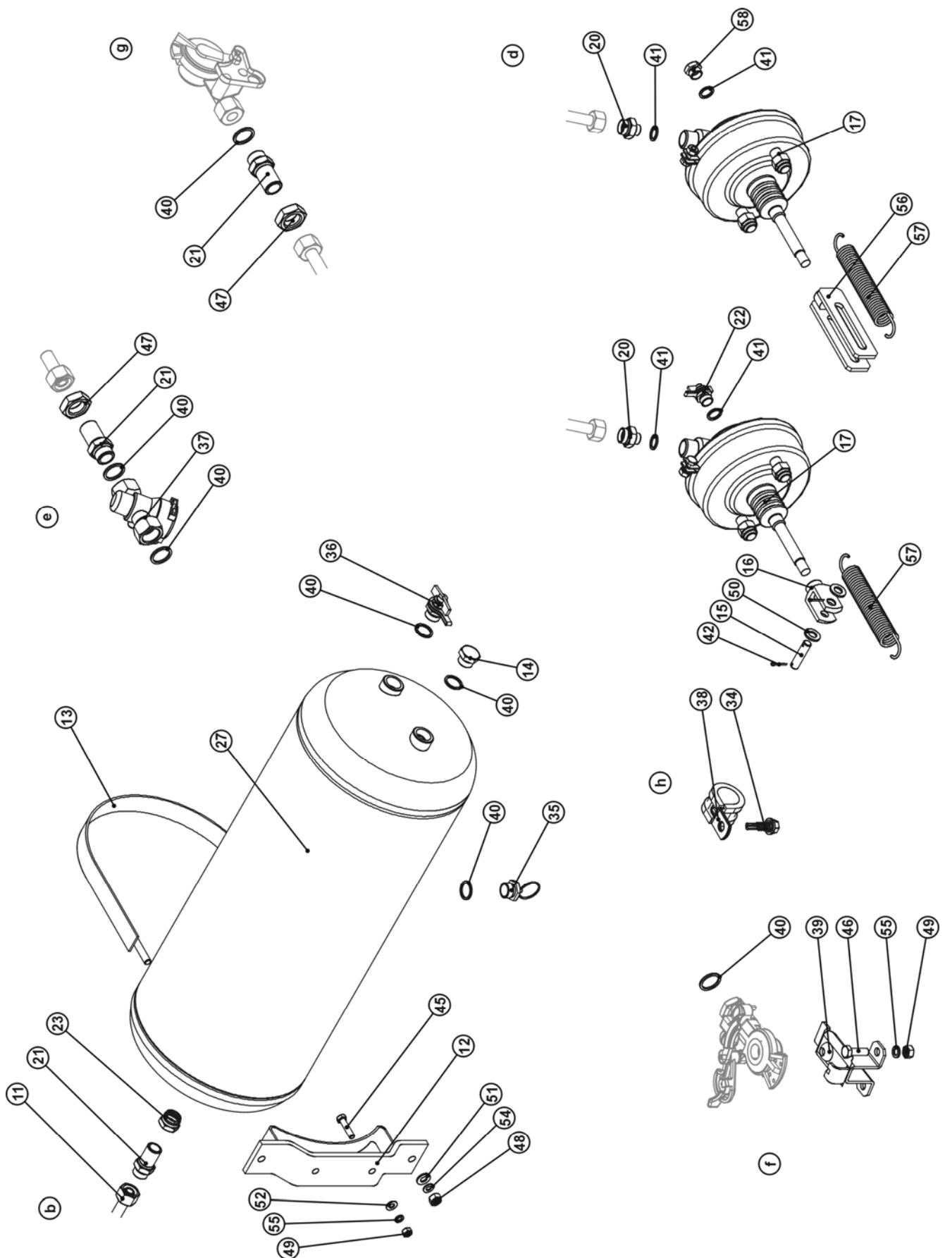
FIG. 8. PNEUMATIC BRAKE SYSTEM I WITH AUTOMATED CONTROLLER
