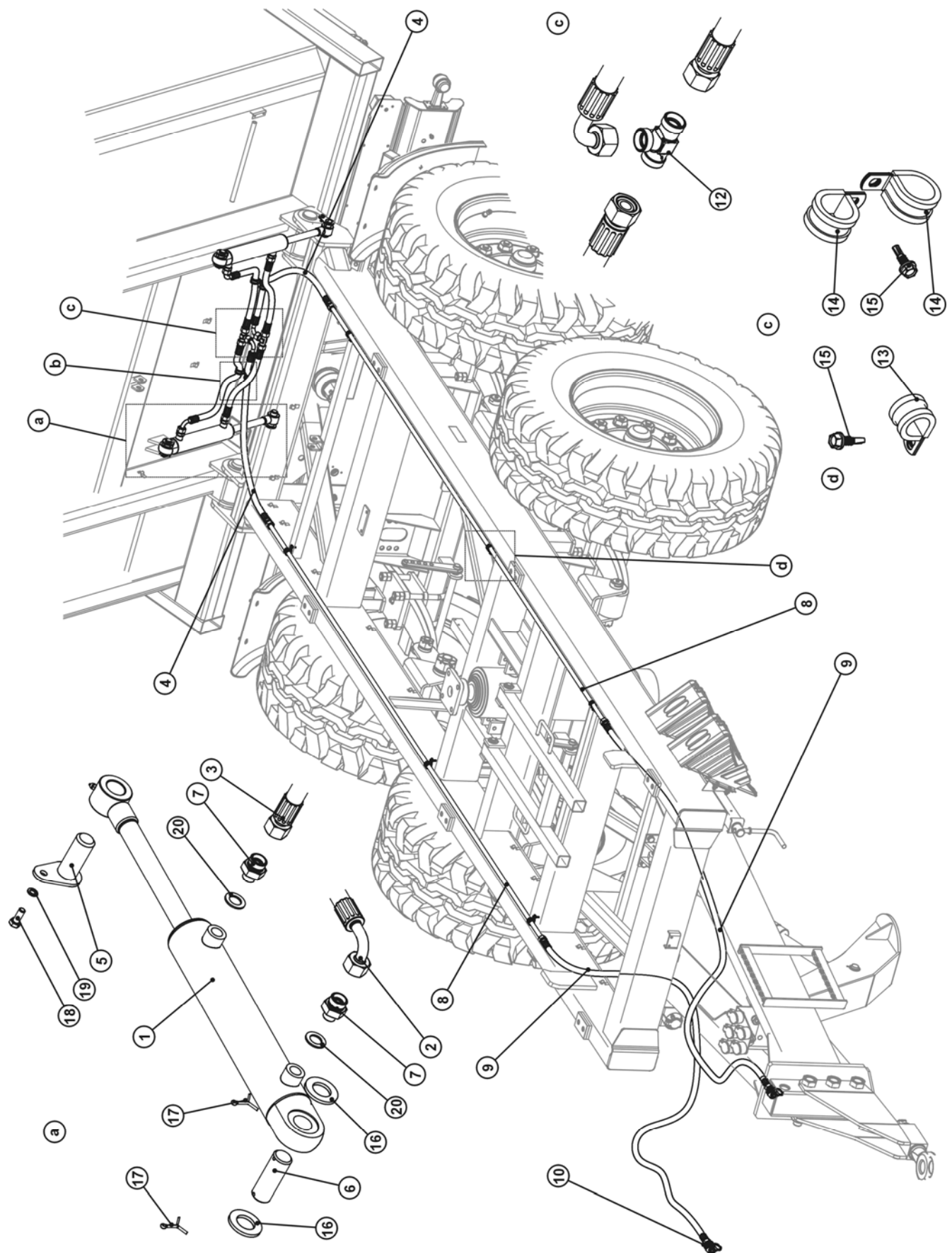
FIG. 37. REAR FLAP HYDRAULIC SYSTEM
