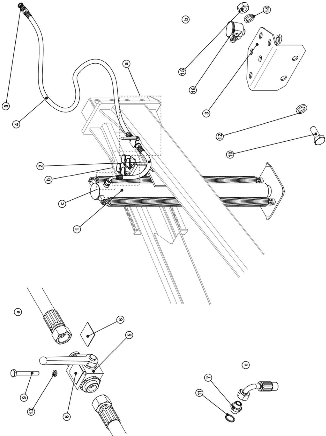
FIG. 27. STRAIGHT SUPPORT HYDRAULIC SYSTEM
