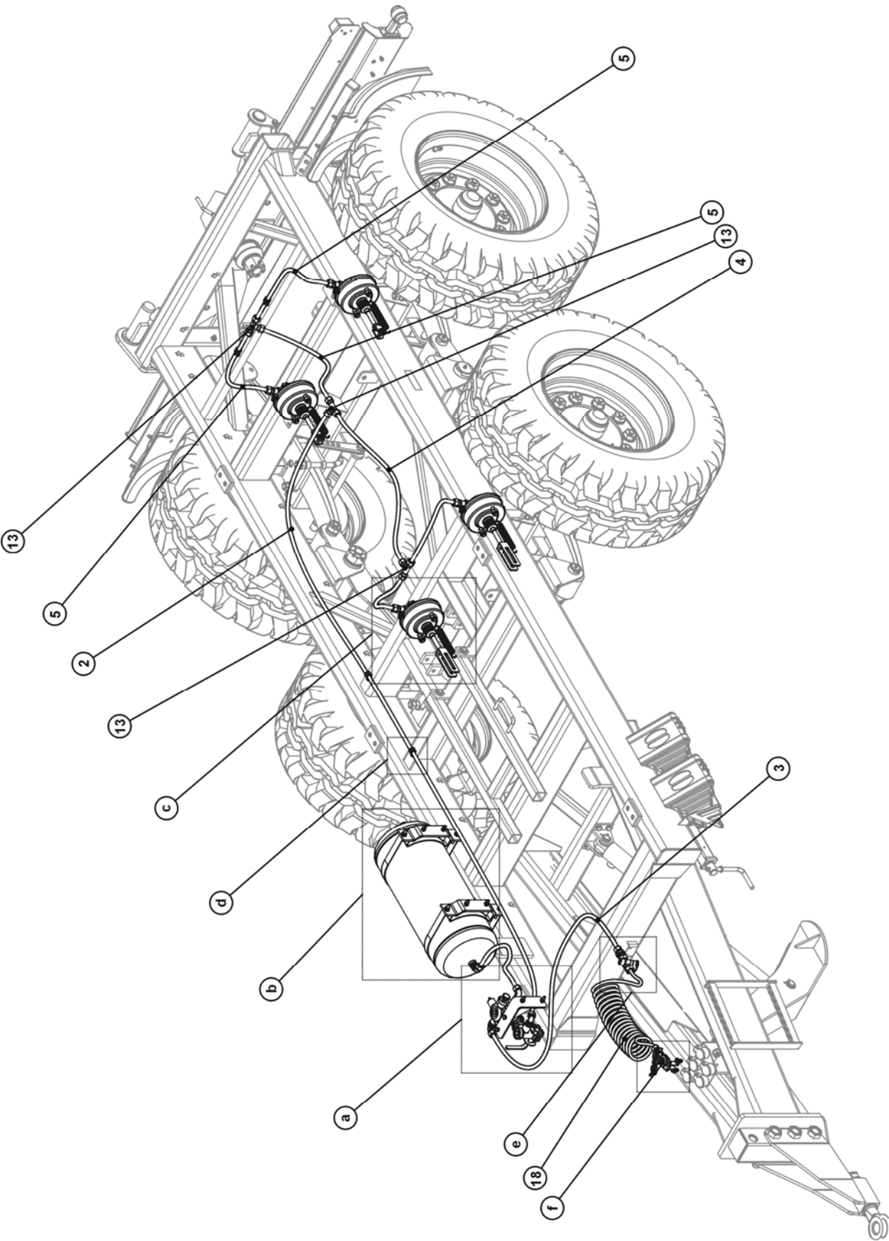
FIG. 22. SINGLE-CONDUIT PNEUMATIC BRAKE SYSTEM II WITH THREE-RANGE CONTROLLER
