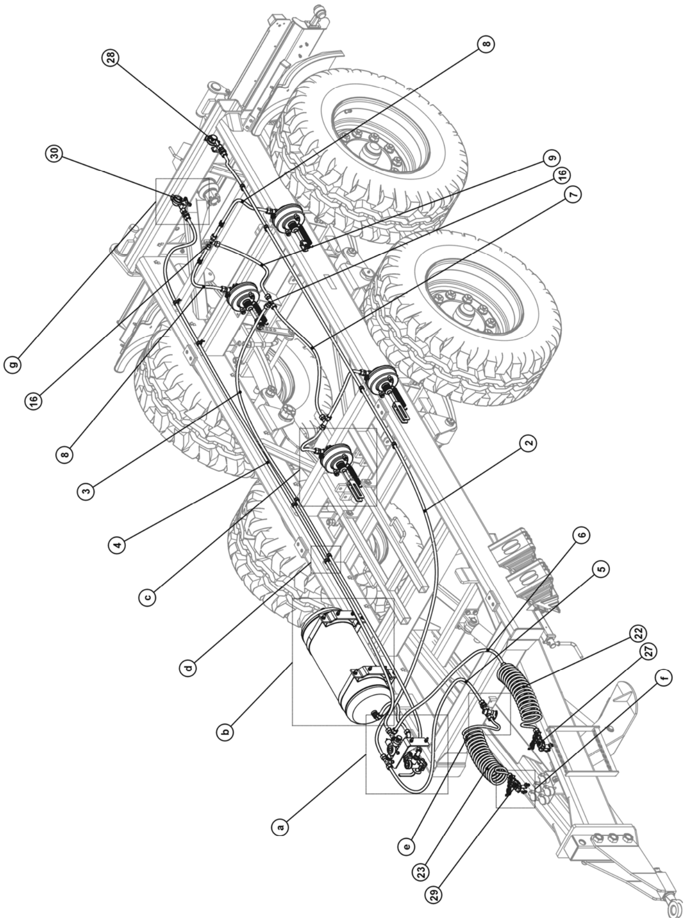
FIG. 13. DOUBLE-CONDUIT PNEUMATIC BRAKE SYSTEM I WITH THREE-RANGE CONTROLLER
